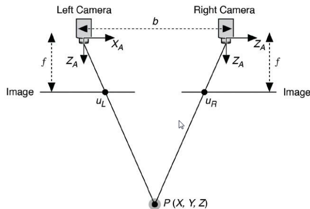
Fig. 10.2: Geometric model of stereo vision. Two calibrated cameras with baseline b observe a 3D point P(X,Y,Z) , which projects to pixel coordinates u_L and u_R in the left and right images, respectively. [Tech Briefs, 2012]
